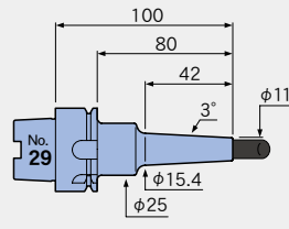
A40-SLFB8-90-M42
