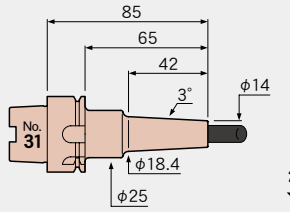
A40-SLRA8-85-M42
