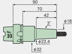
A40-SLFB8-90-M42
